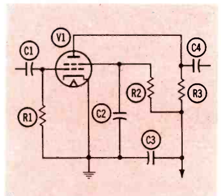
Fig. 2. Grounding in an amplifier stage.
