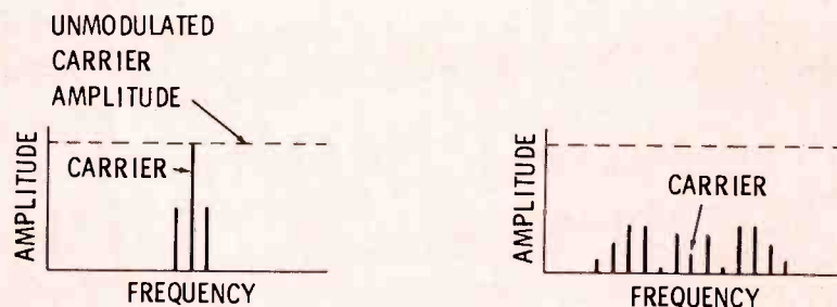
Fig. 2. The sideband composition varies greatly with the method of modulation.
