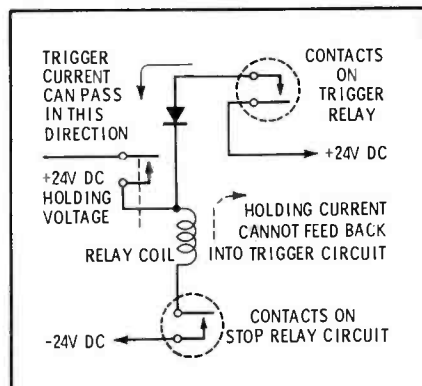
Fig. 3. Diode serves as gate to keep equipment voltage from trigger bus.
