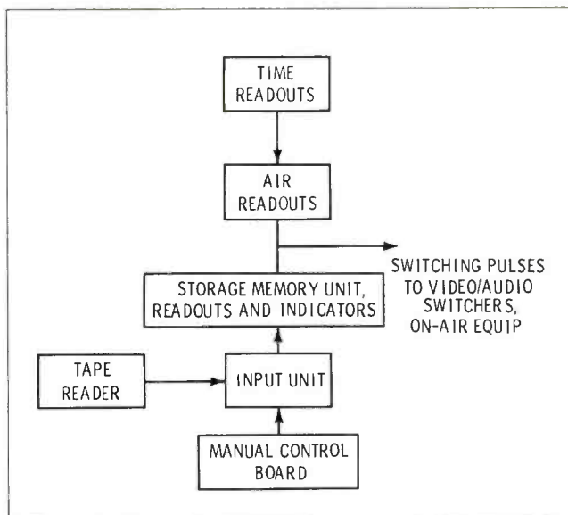
Fig. 6. Block diagram of tape-programmed automation unit.
