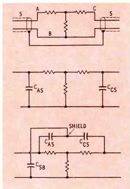
Fig. 8. Frequency distortion is reduced.
