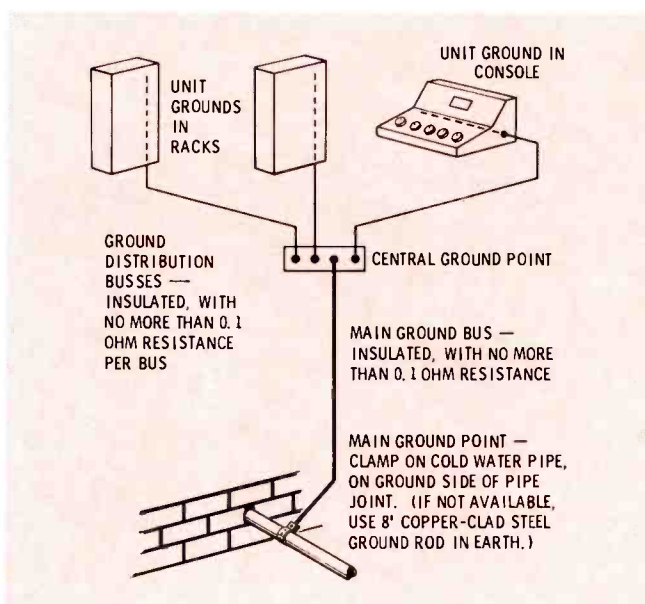
Fig. 5. Unit ground buses connect to a central ground point.
